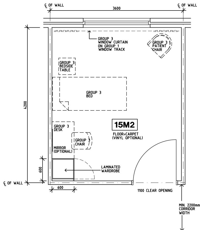
PLAN
