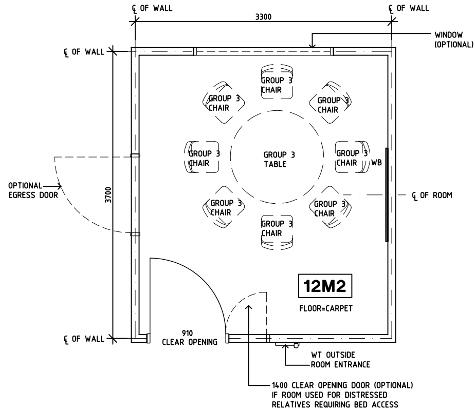
PLAN
