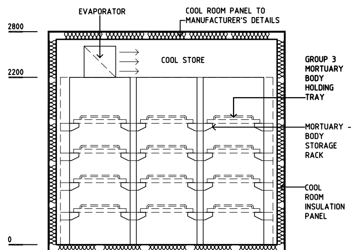
SECTION 5
