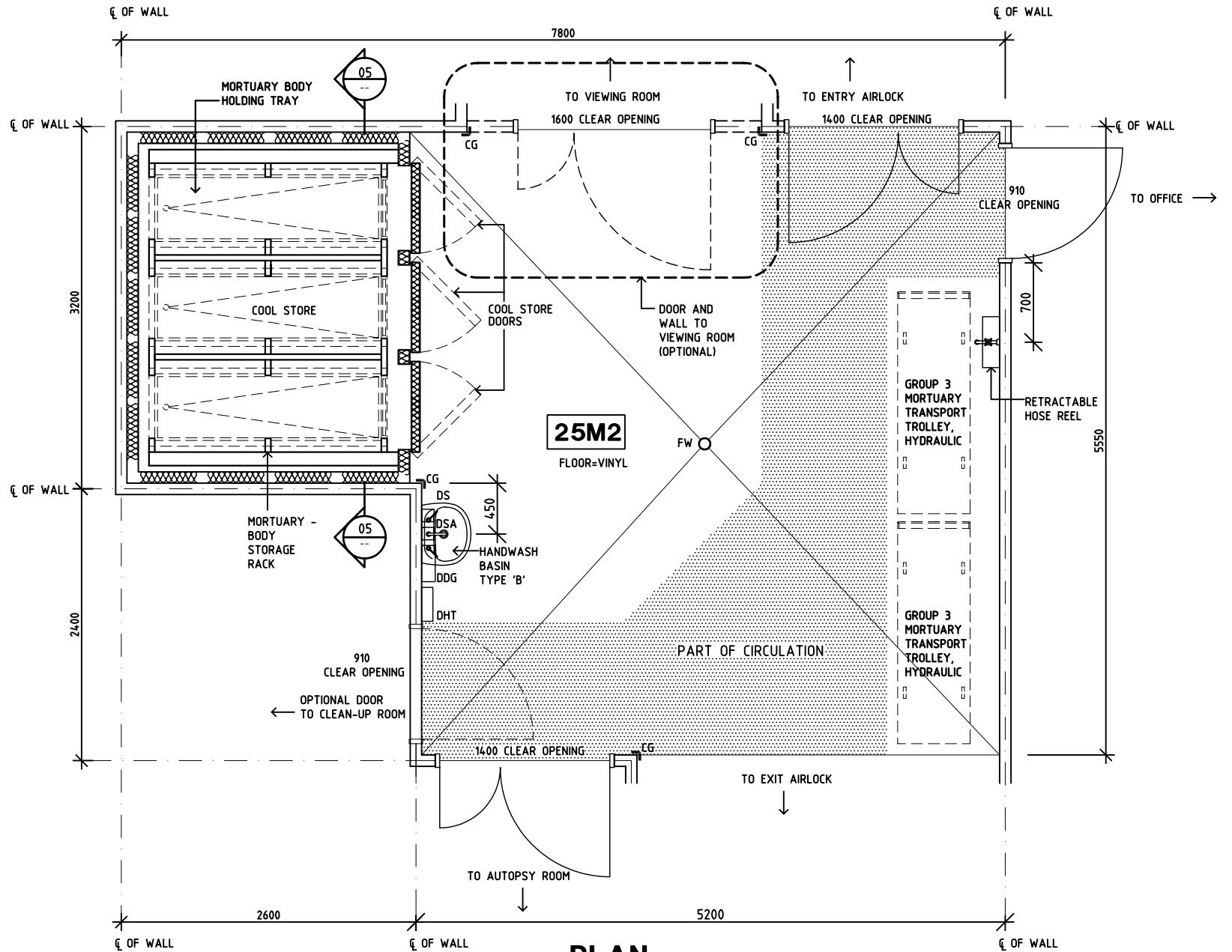
PLAN
