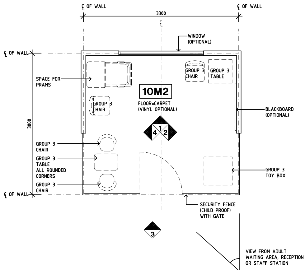
PLAN
