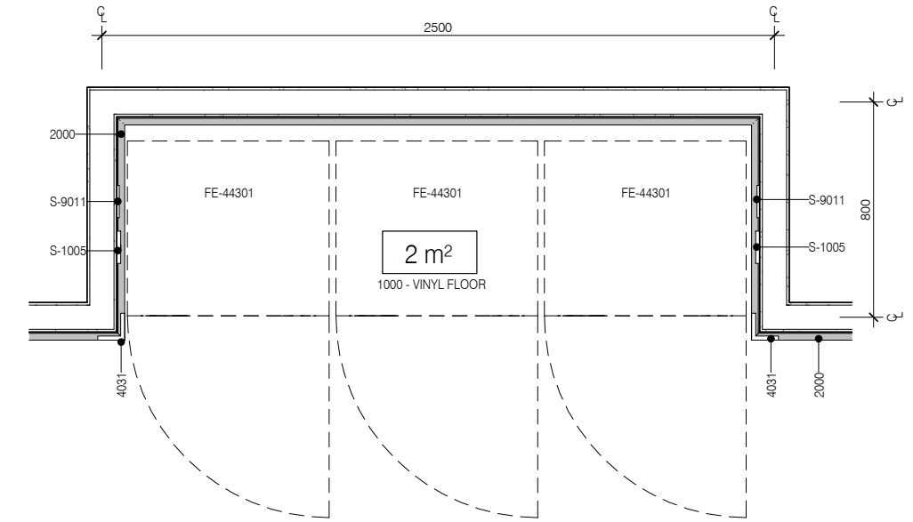
PLAN
