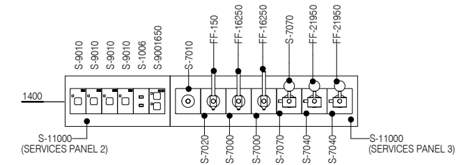
ELEVATION 6 (1 : 25 @ A3)
