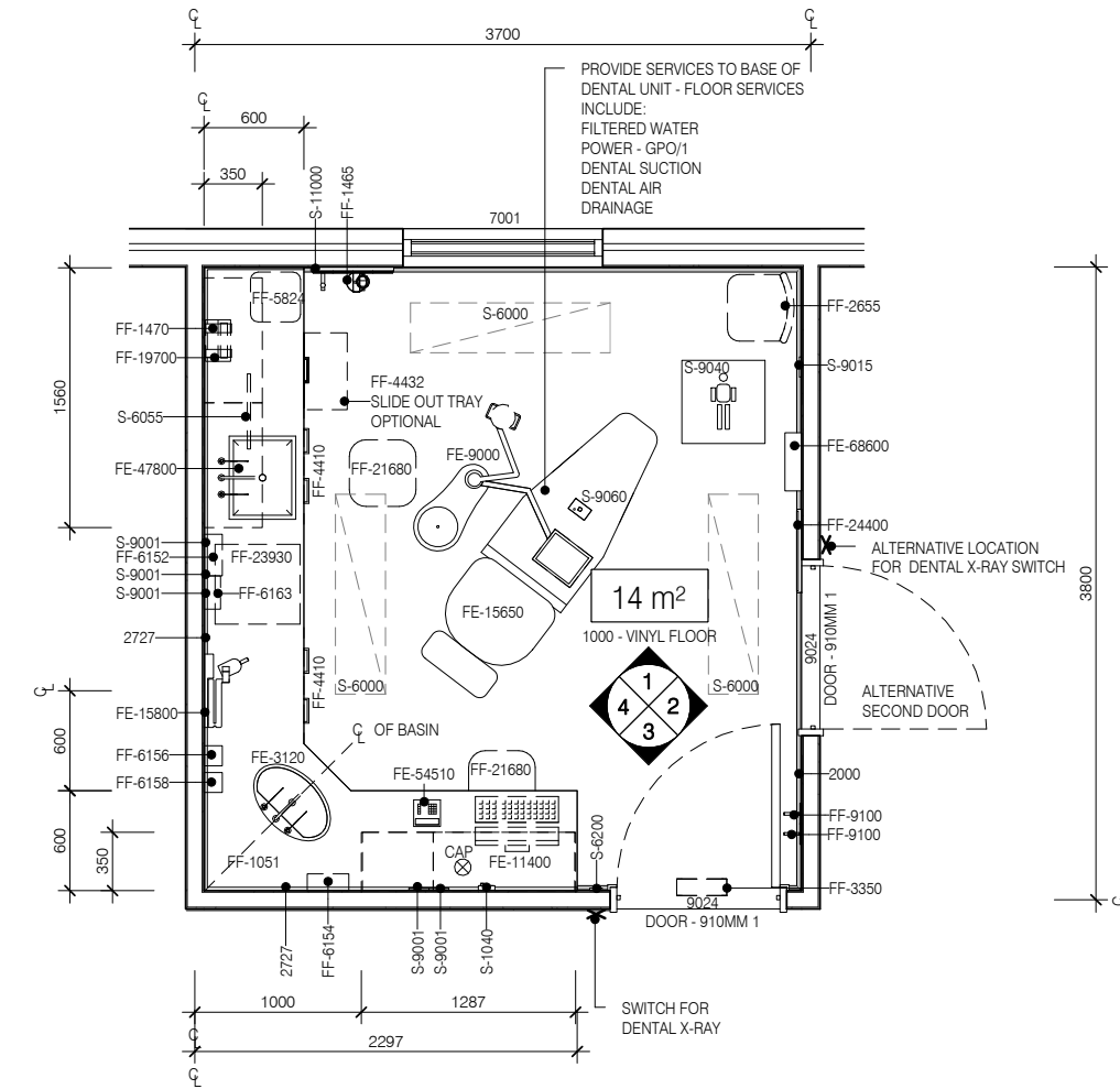
PLAN
