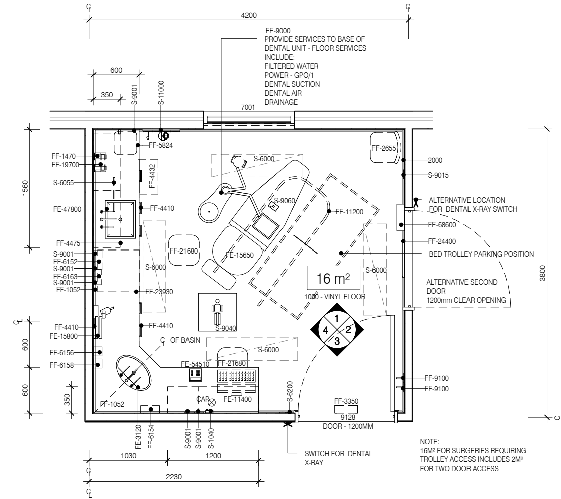
PLAN
