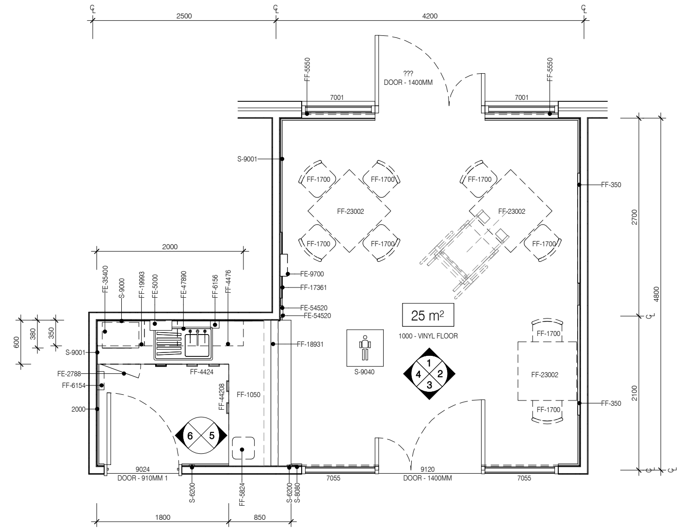
PLAN
