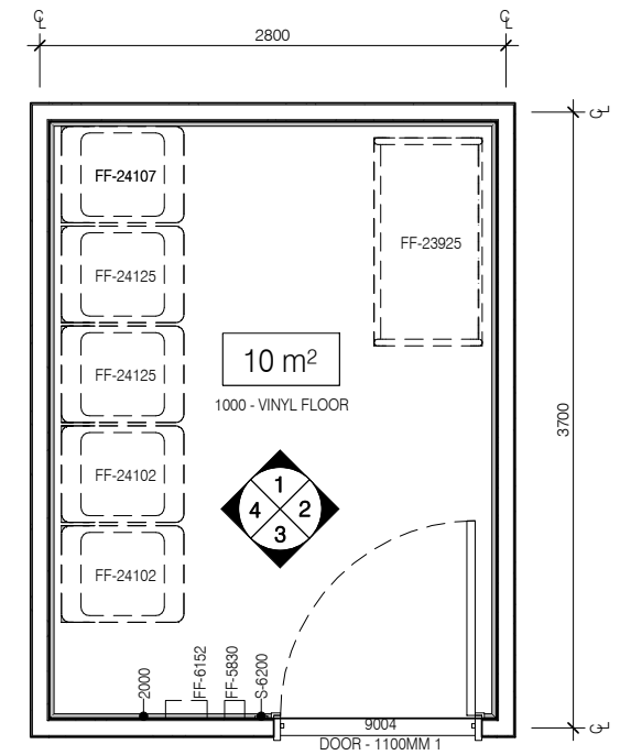
PLAN
