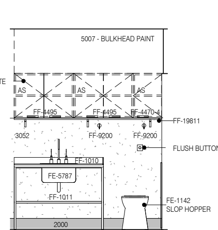
ELEVATION 2 (ALTERNATIVE)
