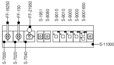
ELEVATION 7 ( 1 : 25 @ A3 )
