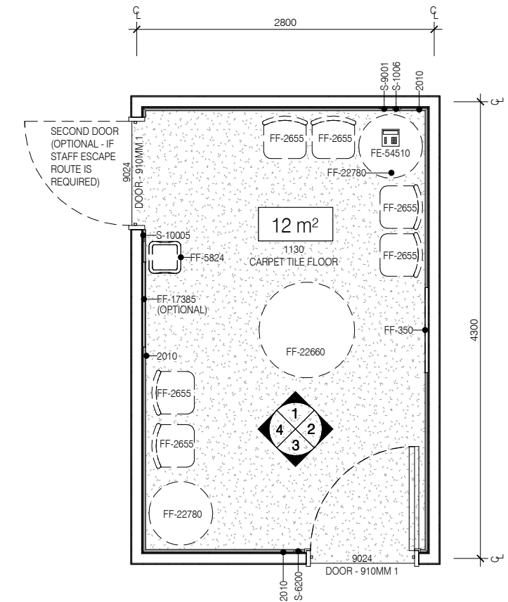
PLAN
