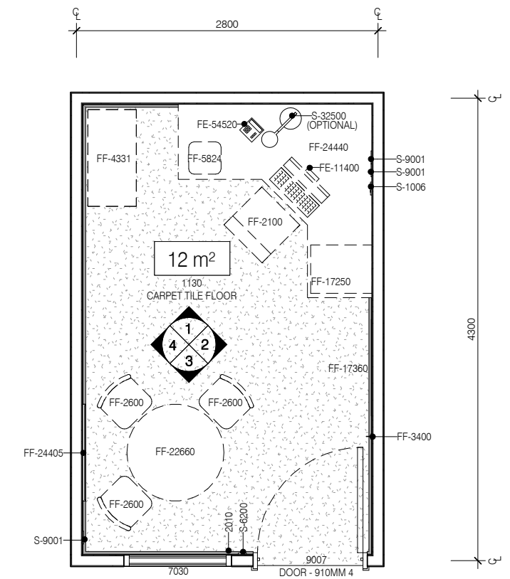
PLAN
