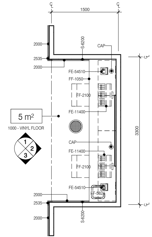
PLAN
