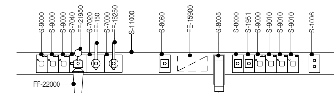
ELEVATION 5 ( 1 : 25 @ A3 )
