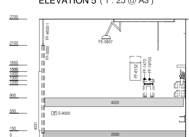
ELEVATION 5 ( 1 : 25 @ A3 )
