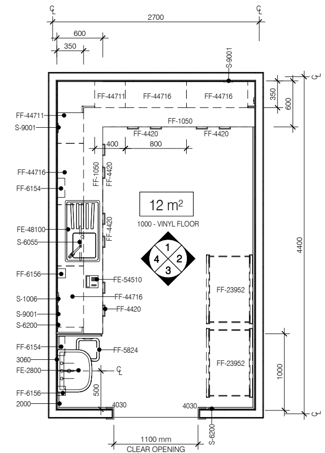
PLAN
