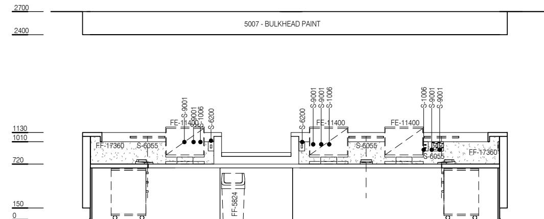
ELEVATION 5 ( 1 : 50 @ A3 )
