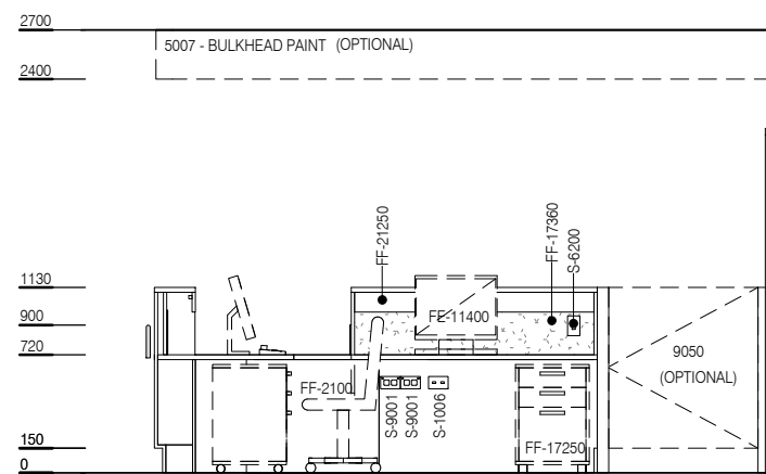
ELEVATION 3 & ELEVATION 4 (MIRRORED)
