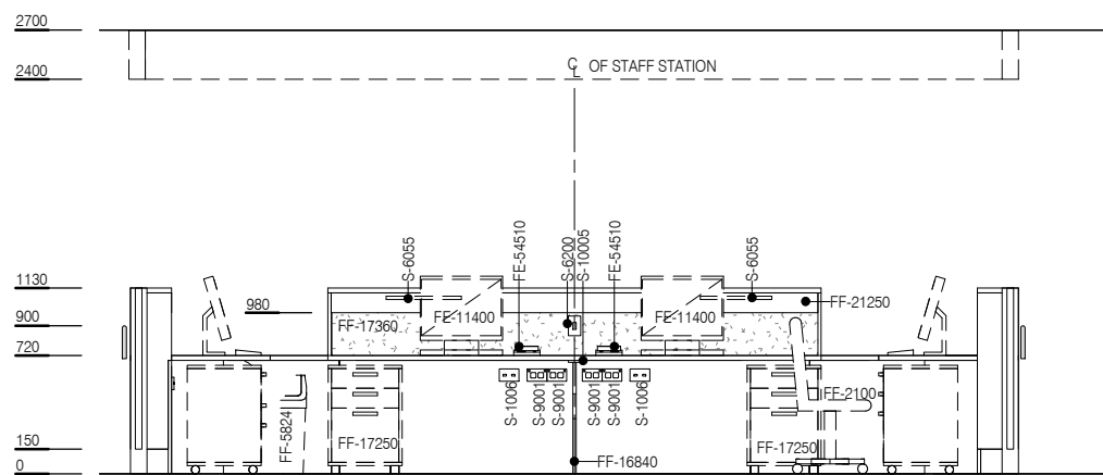
ELEVATION 5 ( 1 : 50 @ A3 )
