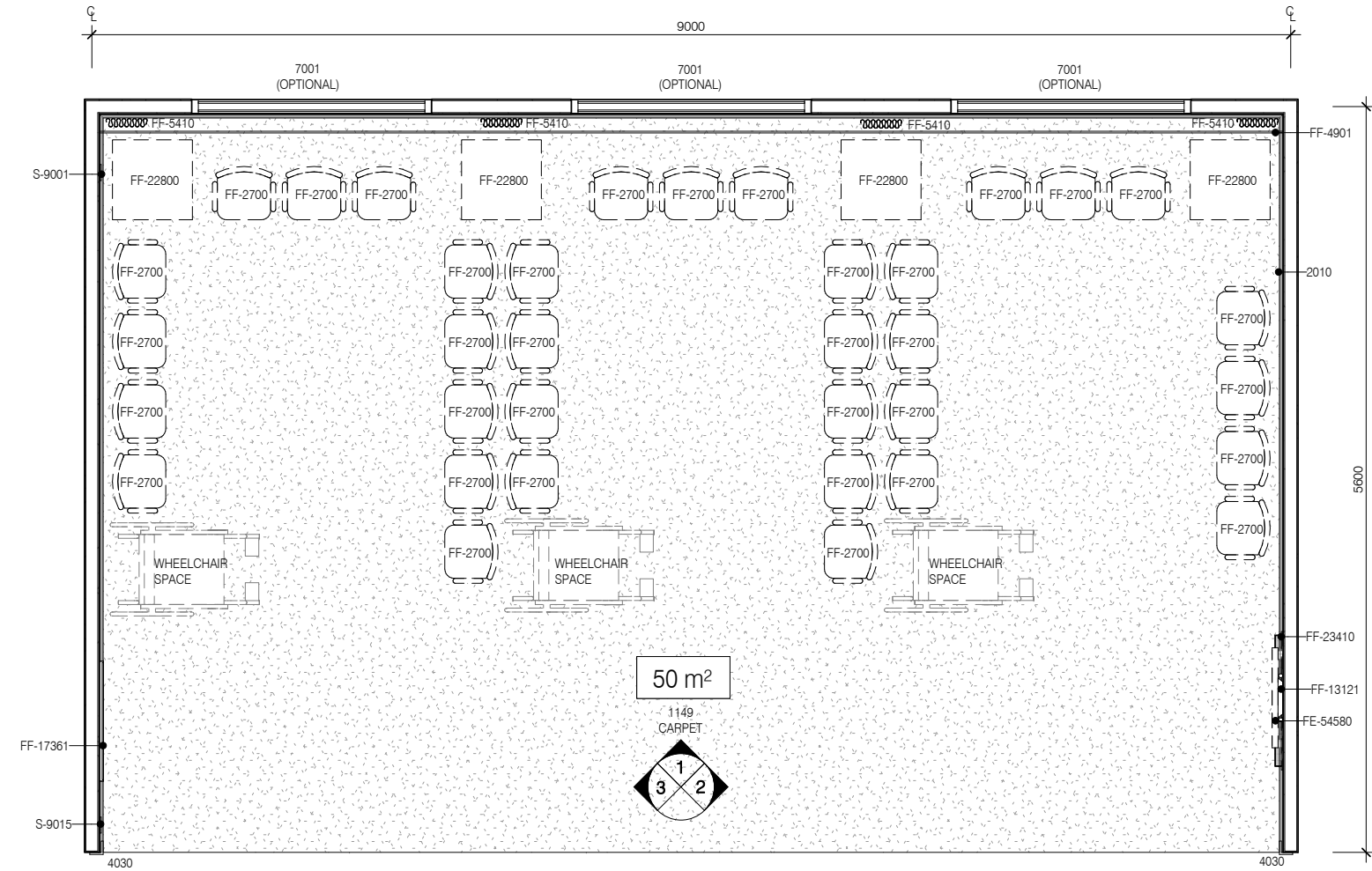
PLAN
