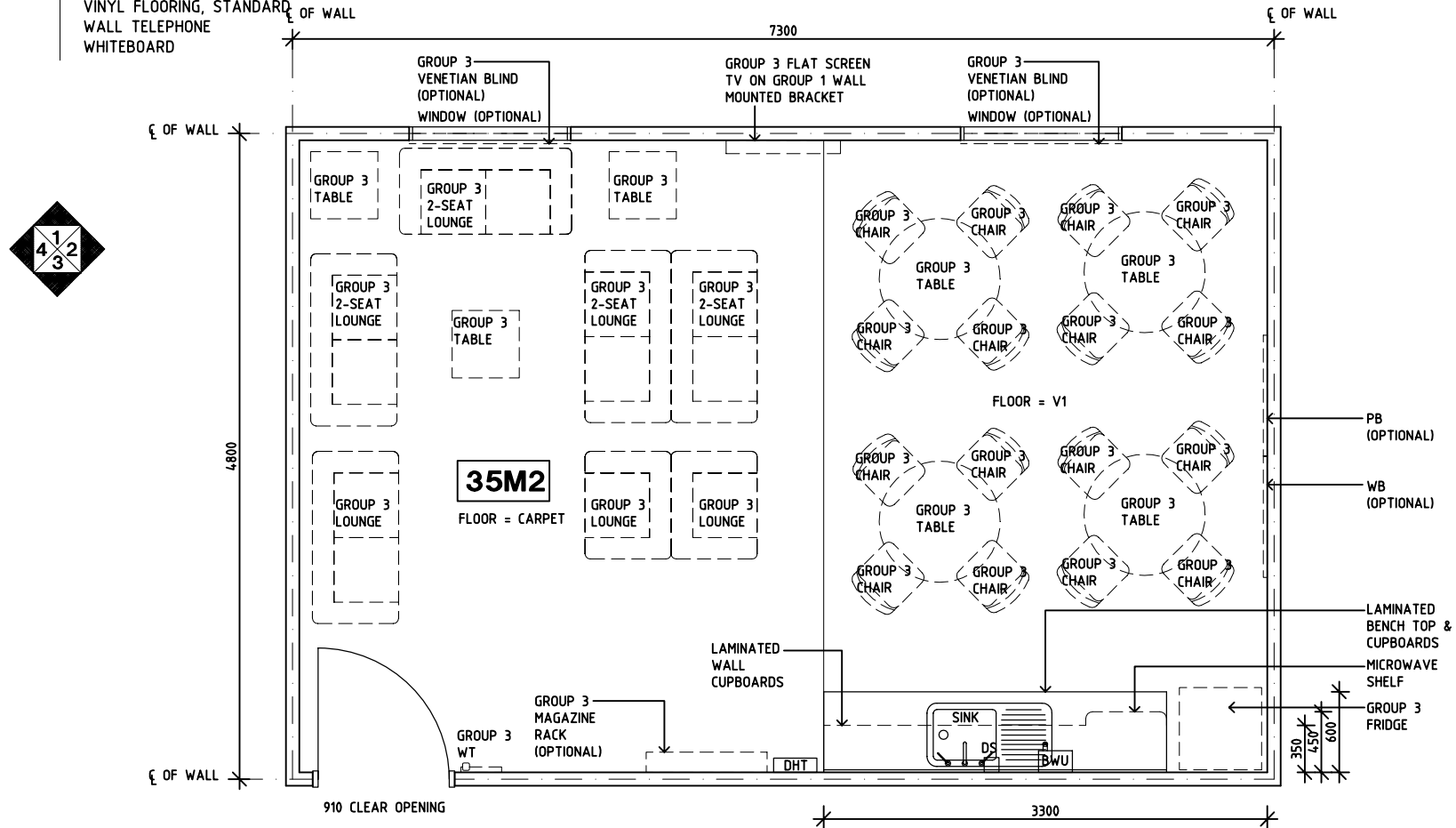
PLAN
