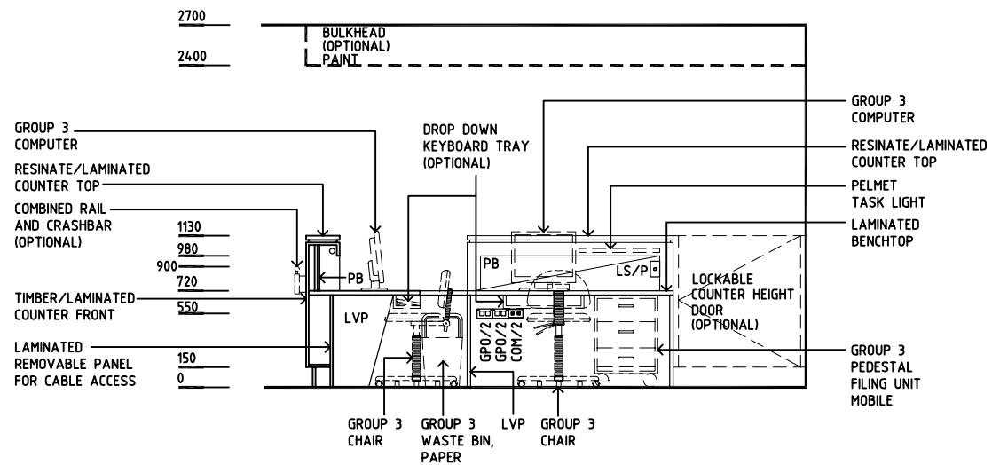
ELEVATION 3 & ELEVATION 4 (MIRRORED)
