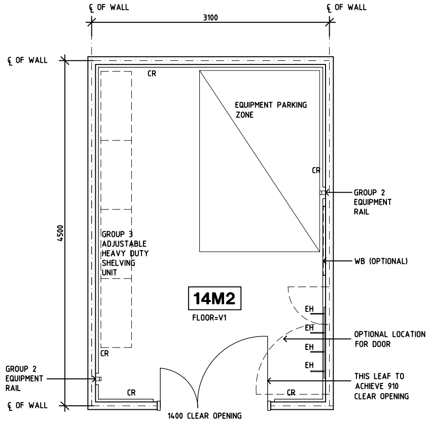
PLAN
