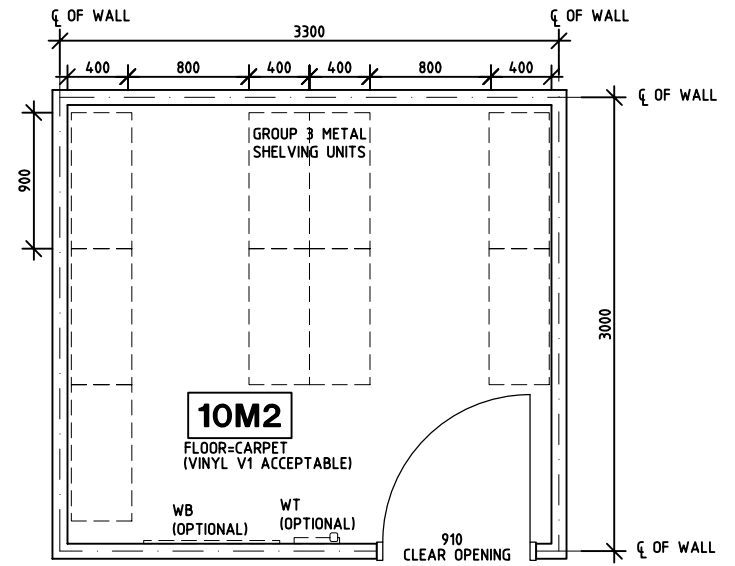
OPTION 2- static shelving PLAN
