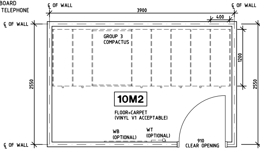
OPTION 1- compactus shelving PLAN
