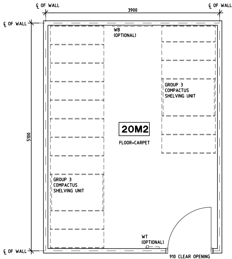
PLAN
