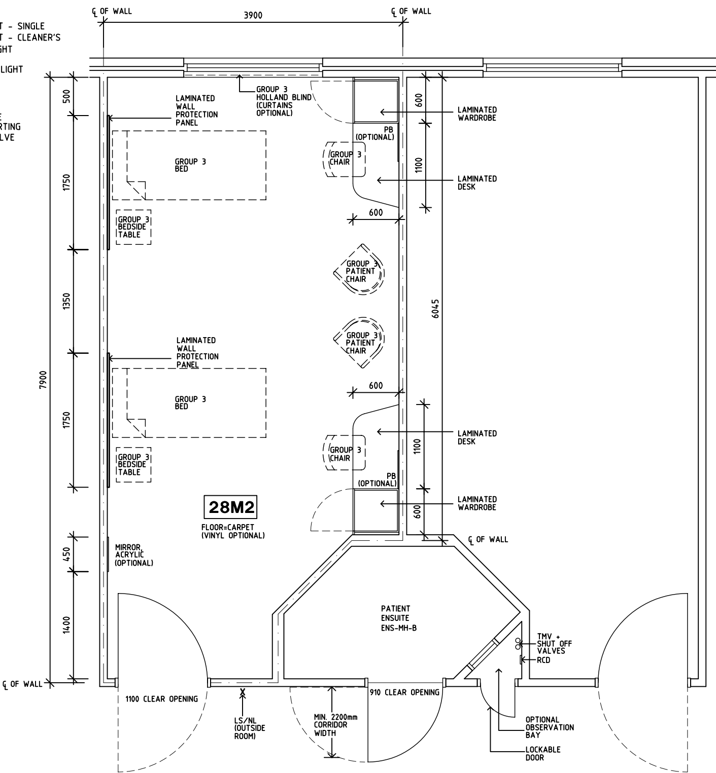
PLAN
