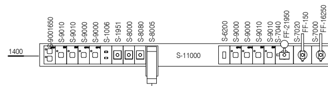
ELEVATION 5 ( 1 : 25 @ A3 )
