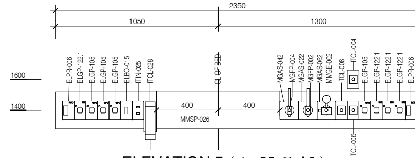
ELEVATION 5 ( 1 : 25 @ A3 )
