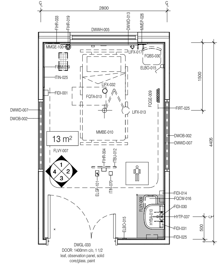
PLAN
