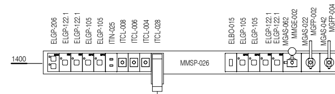
ELEVATION 5 ( 1 : 25 @ A3 )
