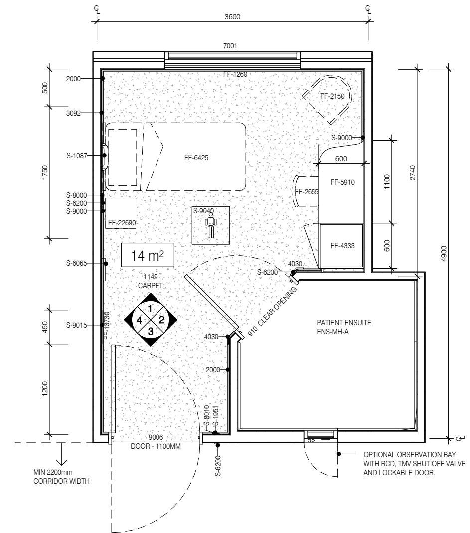
PLAN
