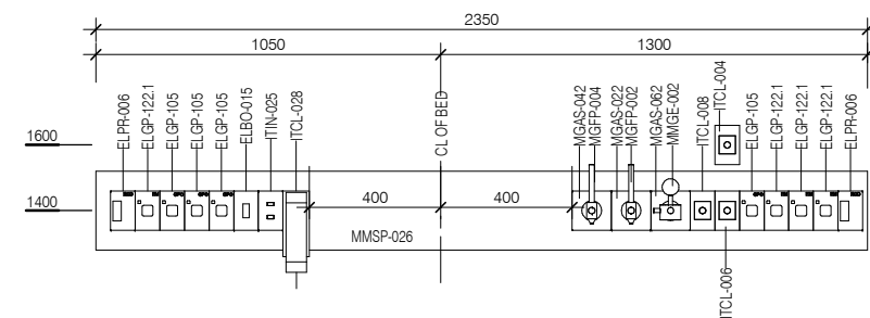
ELEVATION 5 ( 1 : 25 @ A3 )
