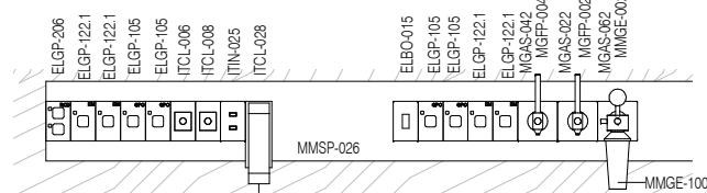
ELEVATION 5 ( 1 : 25 @ A3 )
