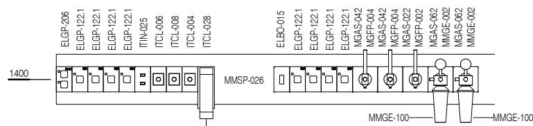
ELEVATION 5 ( 1 : 25 @ A3 )
