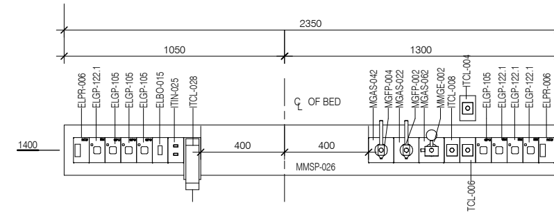
ELEVATION 5 ( 1 : 25 @ A3 )
