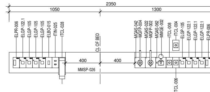
ELEVATION 5 ( 1 : 25 @ A3 )
