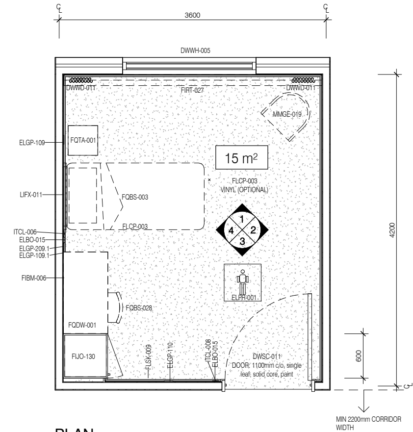
PLAN
