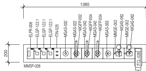
ELEVATION 5 ( 1 : 25 @ A3 )
