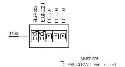
ELEVATION 6 ( 1 : 25 @ A3 )
