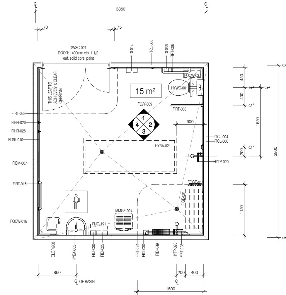
PLAN
