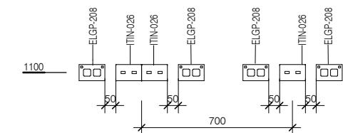
ELEVATION 4 ( 1 : 25 @ A3)
