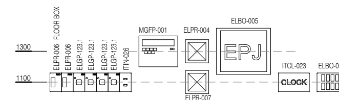
ELEVATION 5 ( 1 : 25 @ A3 )
