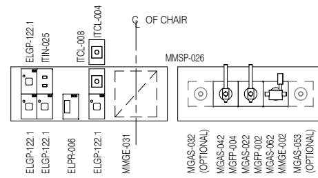
ELEVATION 5 ( 1 : 25 @ A3 )
