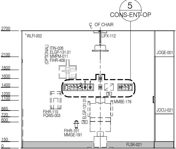
ELEVATION 5 ( 1 : 25 @ A3 )
