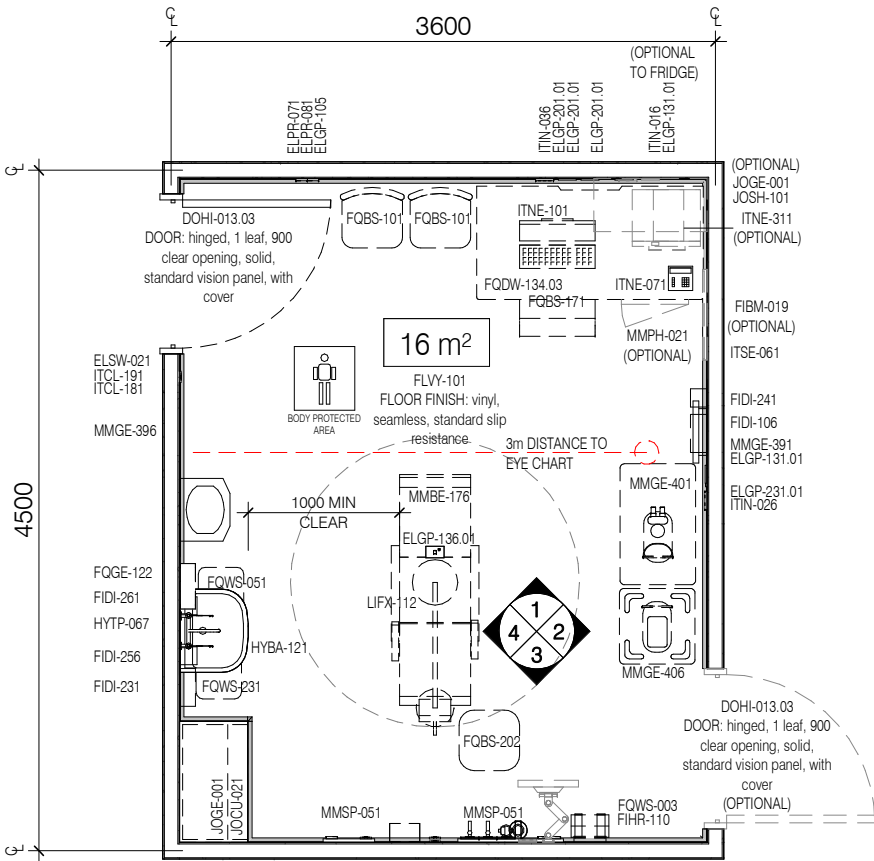
PLAN
