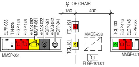
ELEVATION 5 ( 1 : 25 @ A3 )
