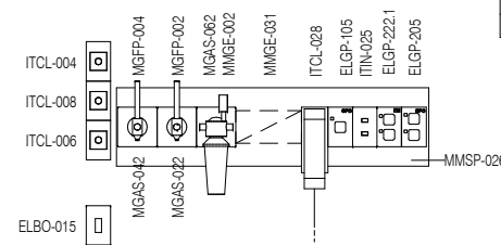
ELEVATION 5 ( 1 : 25 @ A3 )
