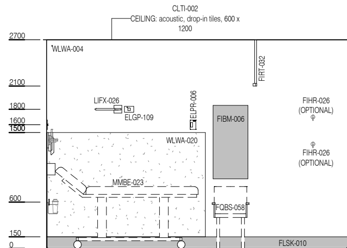
ELEVATION 5 (1 : 25 @ A3)
