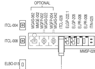
ELEVATION 5 (1 : 25 @ A3)
