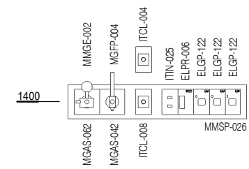
ELEVATION 5 ( 1 : 25 @ A3 )
