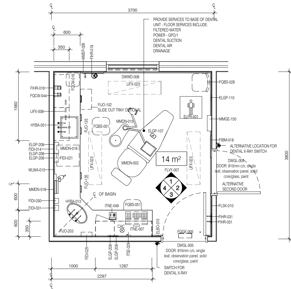
PLAN
