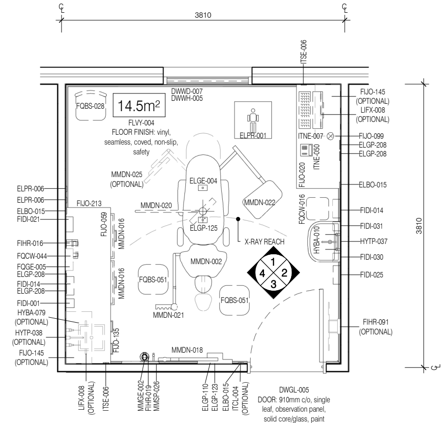
PLAN
