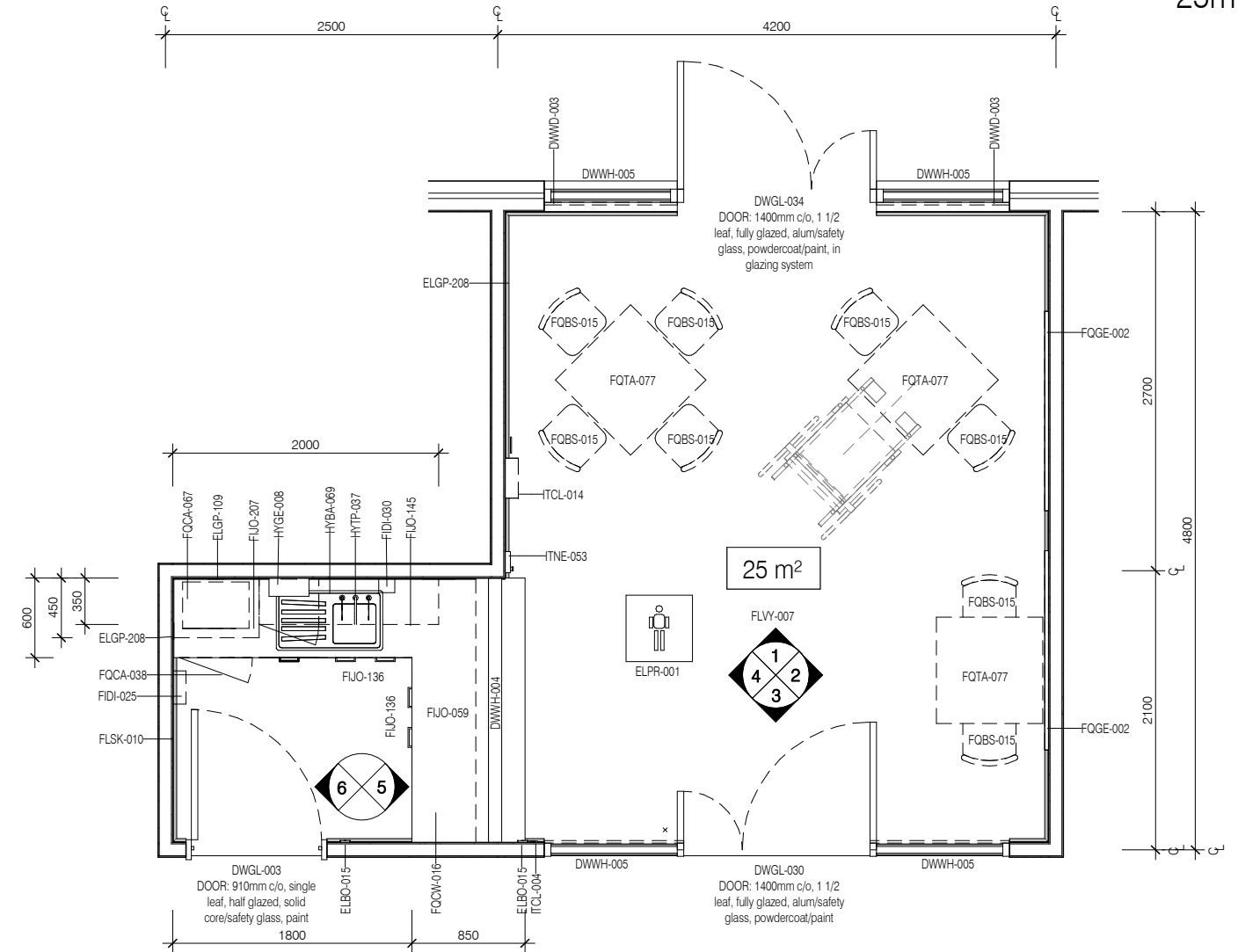
PLAN
