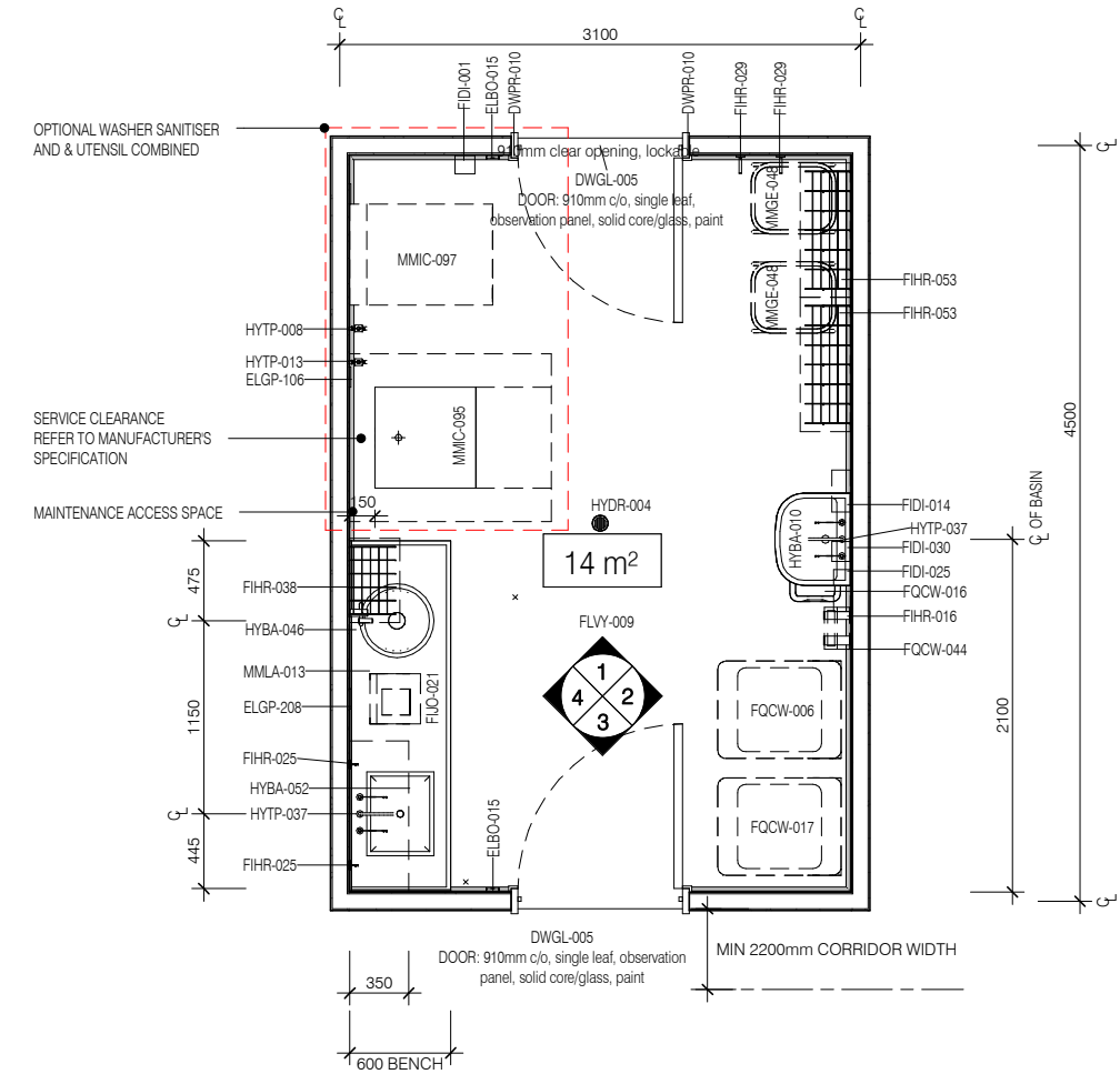
PLAN
